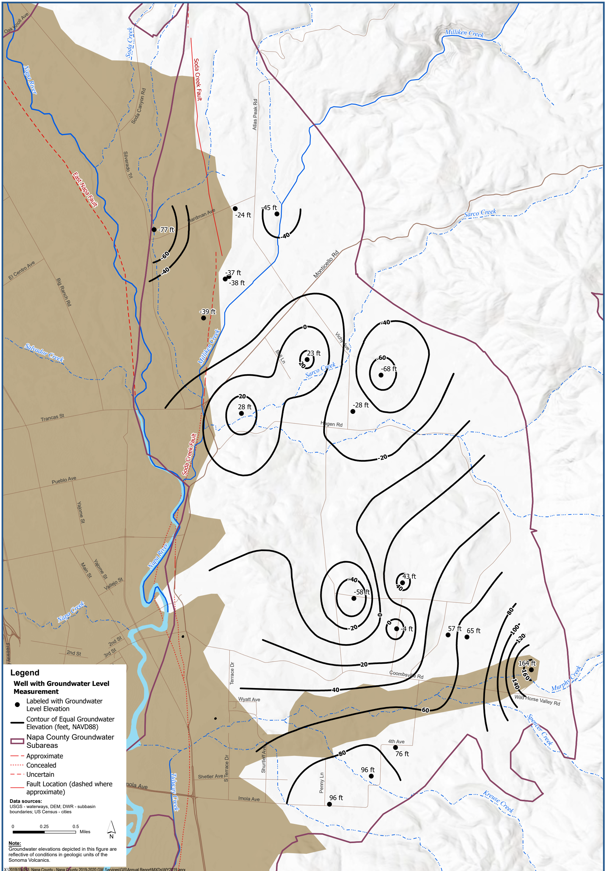
Contours of Equal Groundwater Elevation, Fall 2019 MST Subarea, Napa County, CA Napa County Groundwater Sustainability Annual Report - Water Year 2019
