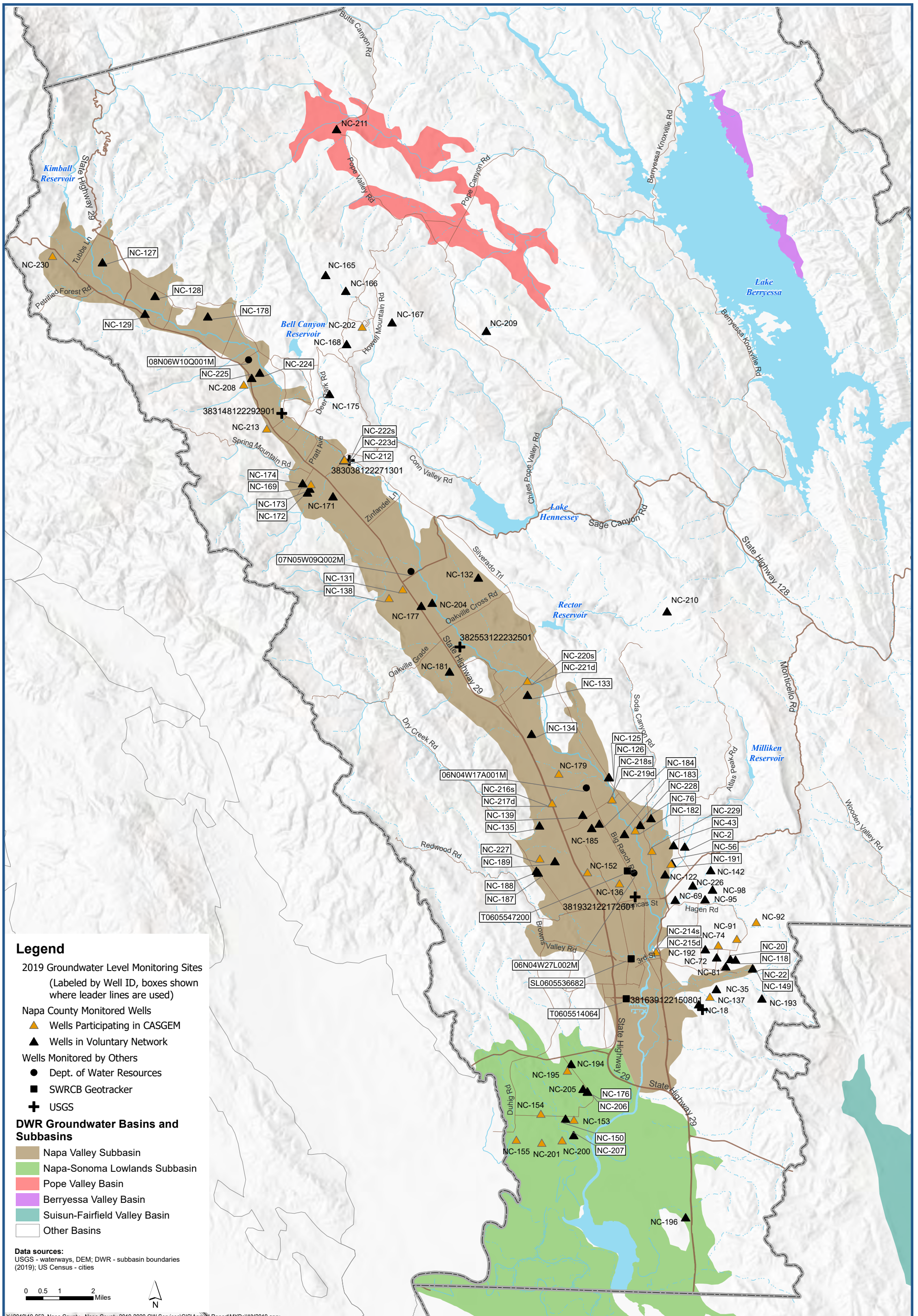
Current Groundwater Level Monitoring Network and CASGEM Sites, Napa County, CA Napa County Groundwater Sustainability Annual Report - Water Year 2019
