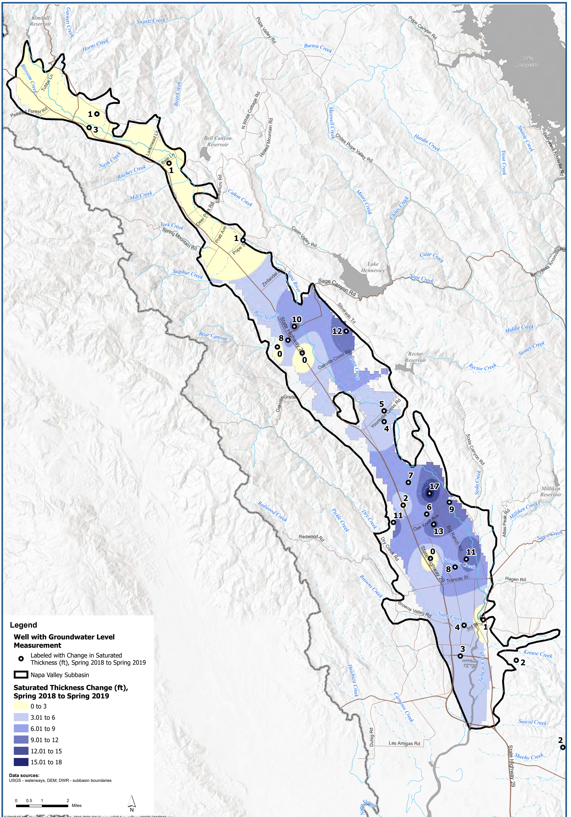
Napa Valley Subbasin Principal Aquifer Change in Saturated Thickness, Spring 2018 to Spring 2019
