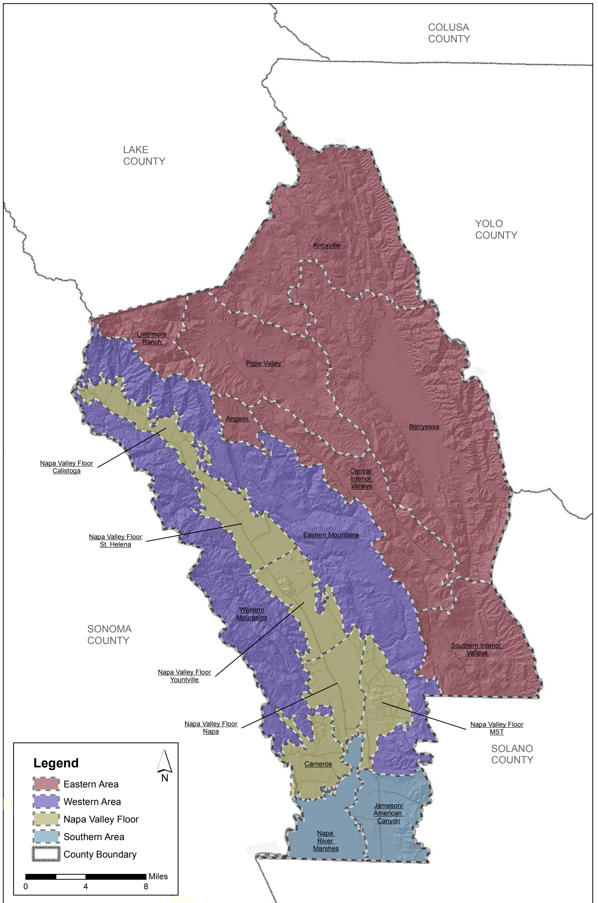
Figure 2.1 Napa County Geologic Areas Napa County, CA
