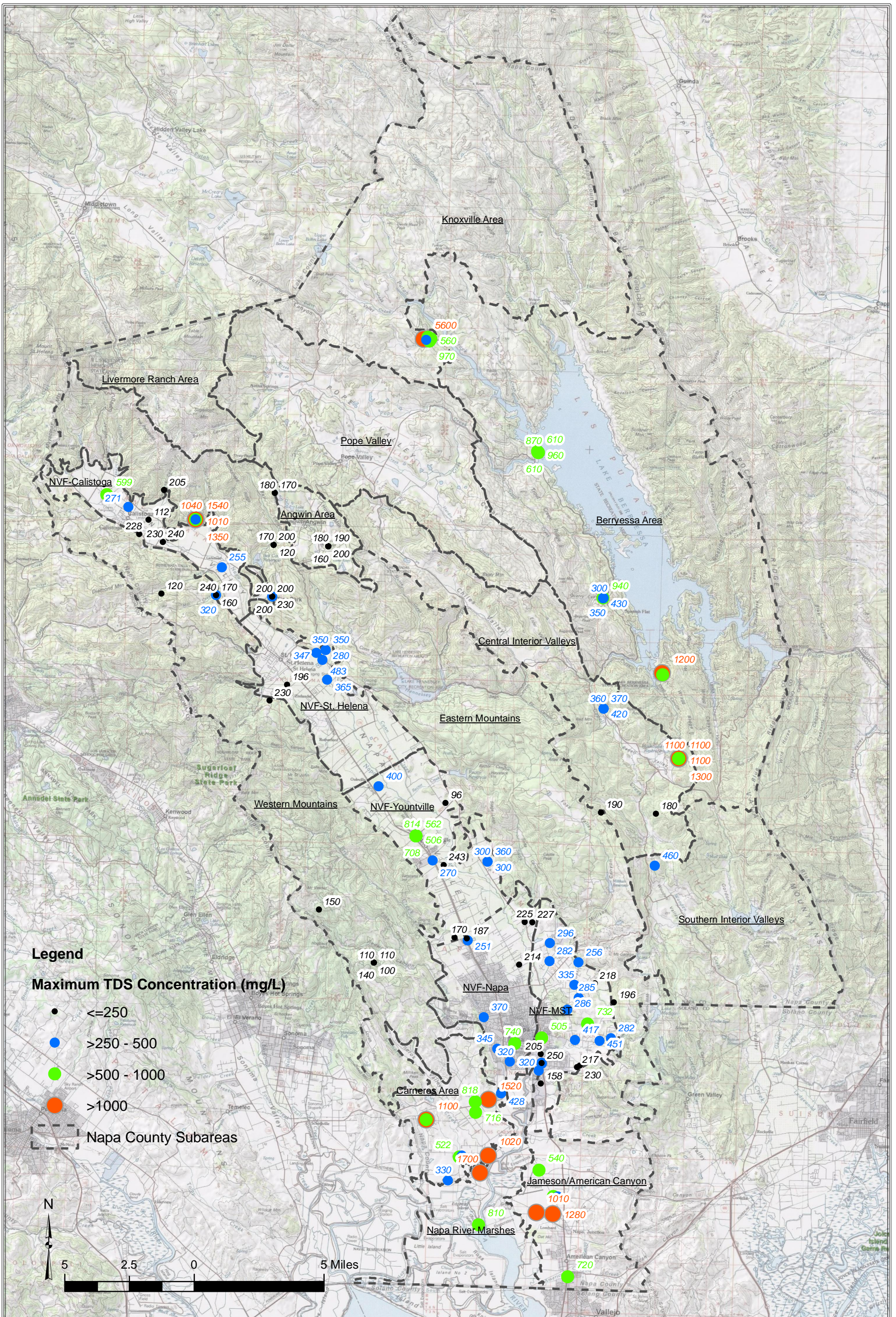
Figure 2.13 Maximum TDS Concentrations Groundwater Quality - Napa County
