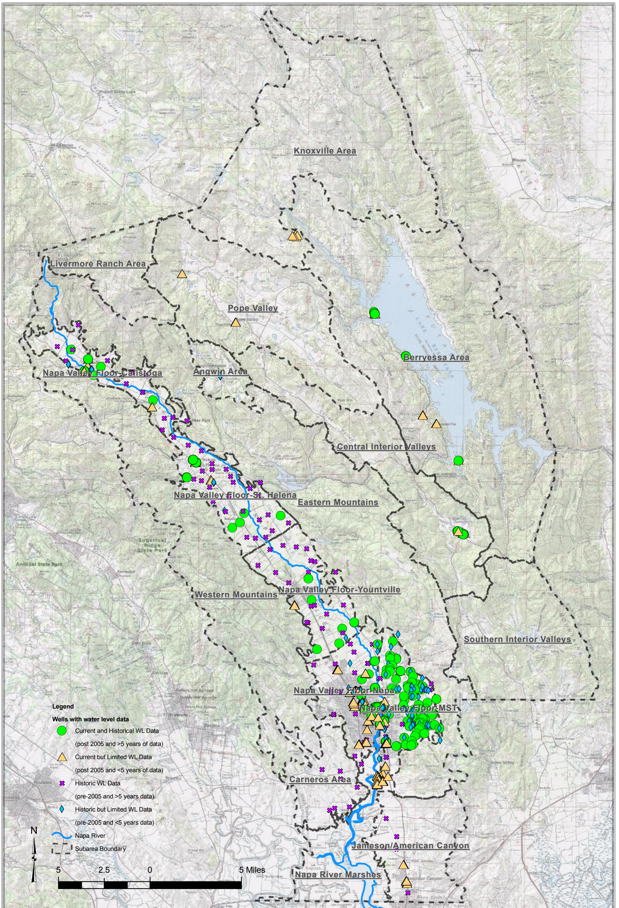
Figure 5.1 Groundwater Level Data Availability
