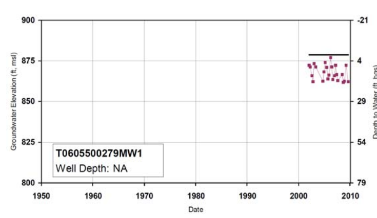
Figure 4.7 Representative Hydrographs for Subareas East of Valley Floor Groundwater Elevations - Napa County
