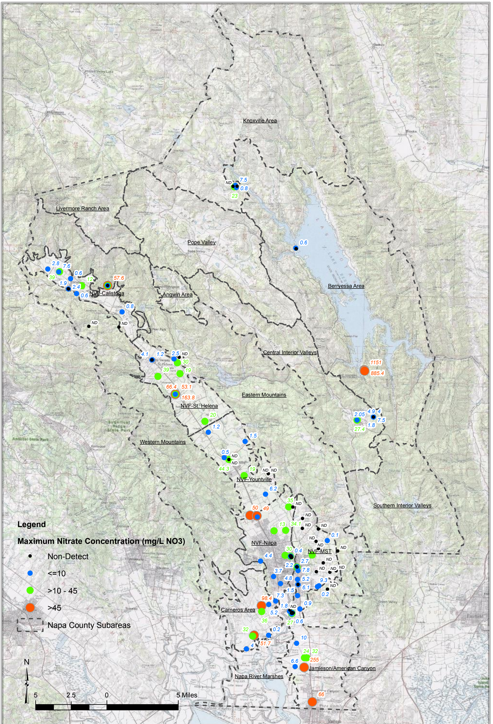
Figure 4.22 Maximum Nitrate Concentrations Groundwater Quality - Napa County
